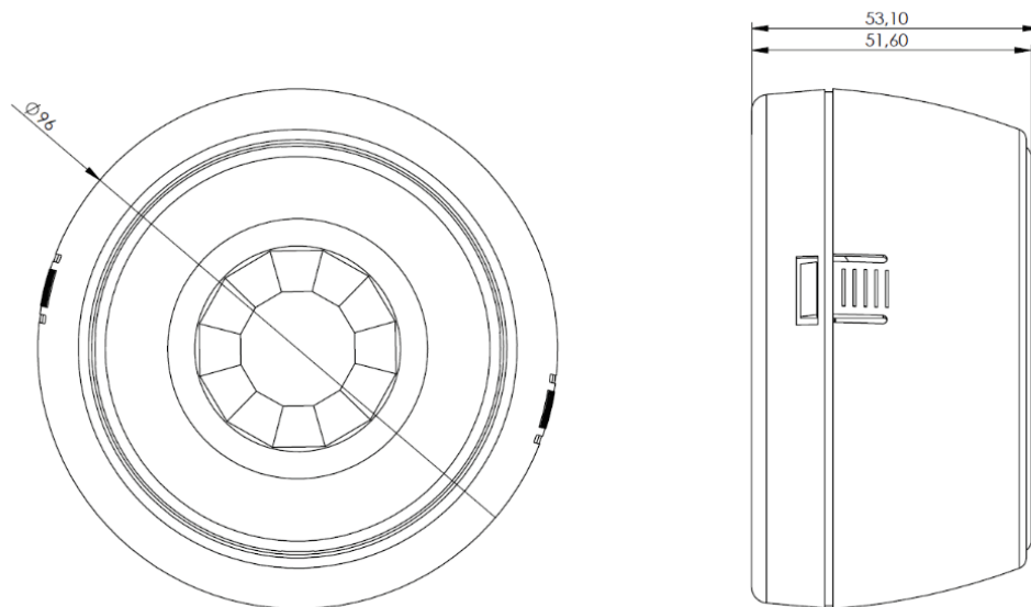
Drawing 1: Surface Mount
