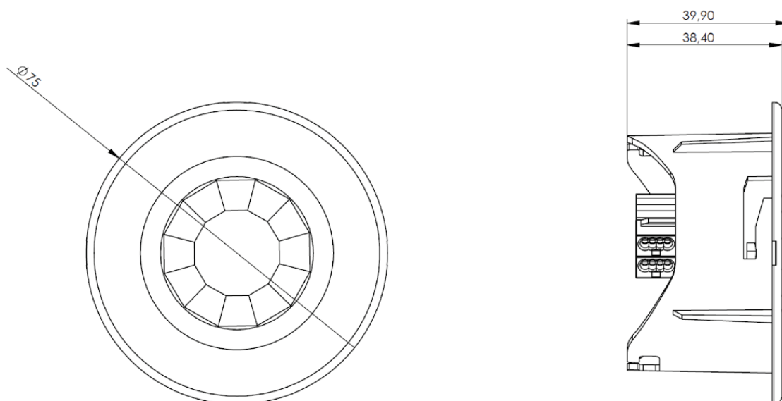
Drawing 2: Flush Mount
